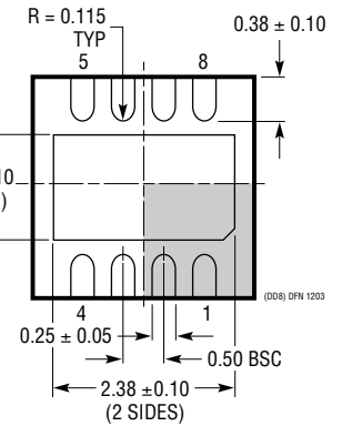
BOTTOM VIEW—EXPOSED PAD
