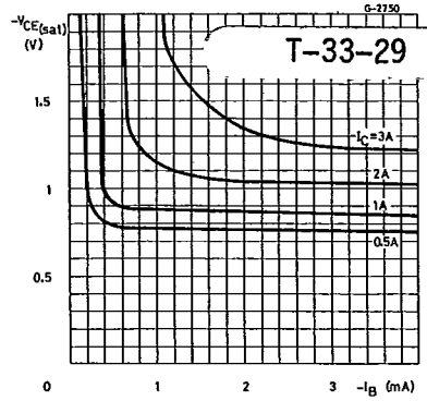
Collector-emitter Saturation Voltage (PNP).
